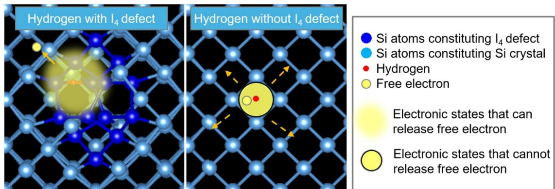
Schematic of free electron generation from hydrogen via the synergistic interaction with the defect
